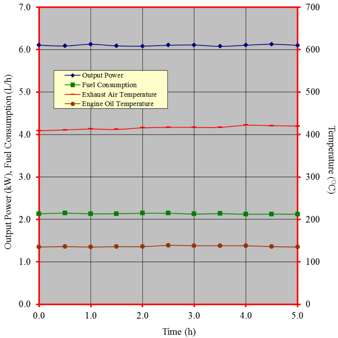
Figure 4. Performance characteristic curves during the continuous running test of the KOHLER KD440 diesel engine
