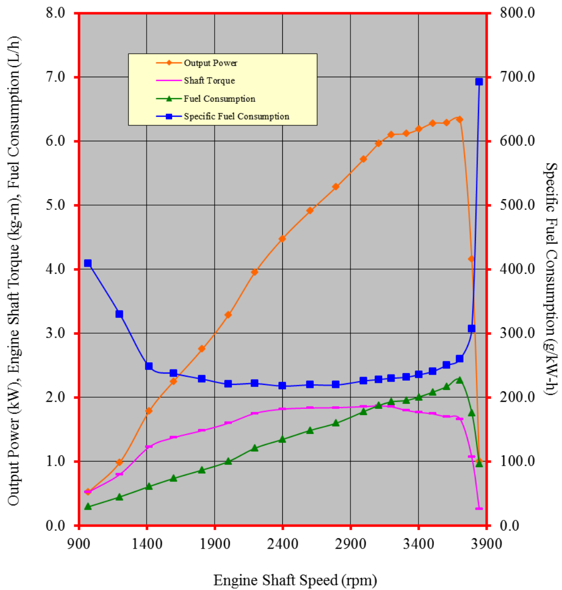
Figure 3. Performance characteristic curves of the KOHLER KD440 diesel engine
